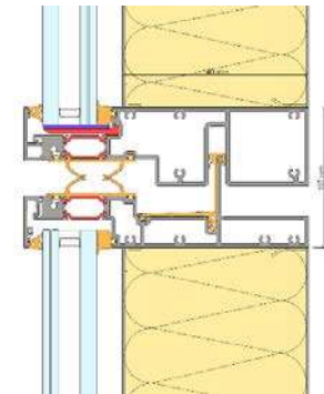
Vertical Section
