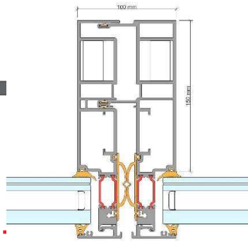
Vertical Section
