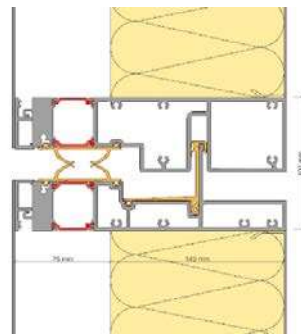
Vertical Section
