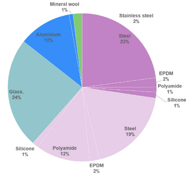
Embodied Carbon by Material (A-C) kgCO 2 eq/m 2
