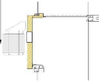
Vertical Section
